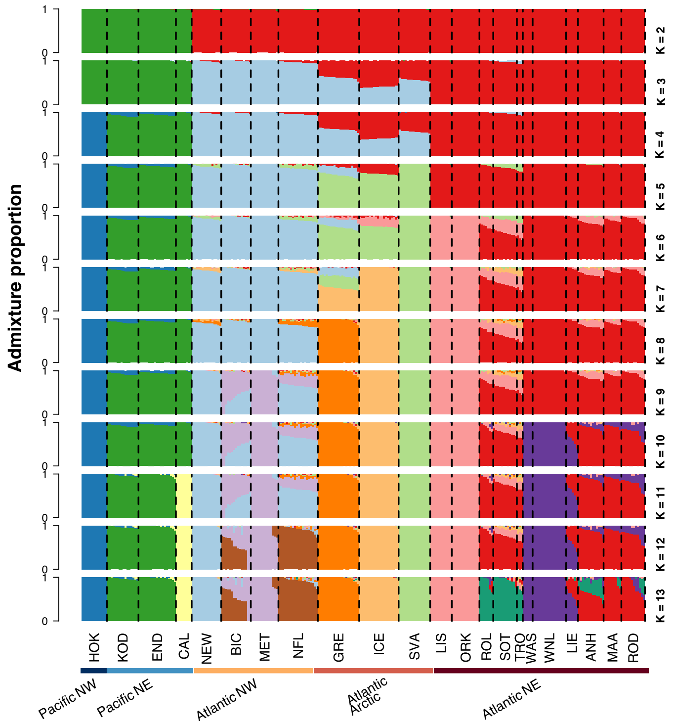
FIGURE 2 Fine-scale genetic structure of global harbour seal populations illustrated by NGSADMIX analysis with assumed number of ancestral populations K ranging from 2 to 13 (convergence was not obtained for any higher K values). Each small vertical bar represents a harbour seal and the colouring corresponds to its genetic ancestry. Locality names and sample sizes are listed in Table S1
