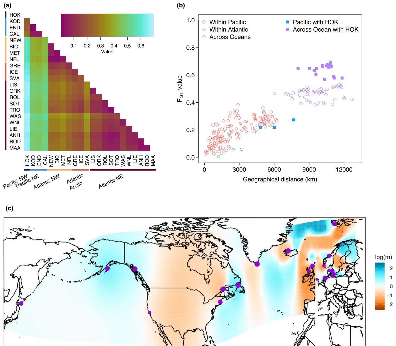
FIGURE 4 The estimates of genetic differentiation indicate a deep genetic split between North Pacific and North Atlantic harbour seal localities and substantial substructure within ocean basins, driven by geographical distance and dispersal barriers. (a) Pairwise F_{ST} estimates among all sample localities; (b) isolation by distance across the harbour seal's range plotted as pairwise F_{ST} estimates among sampling localities against their shortest waterway distance measured in kilometres; (c) dispersal barriers (shades of brown) identified by an EEMS analysis. Locality names and sample sizes are listed in Table S1
